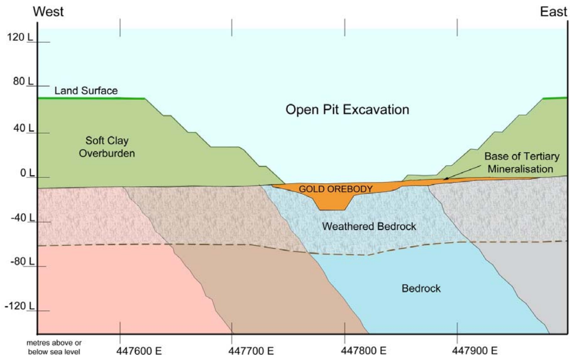
Schematic cross section through proposed Portia open pit designed to recover the base of Tertiary gold mineralisation
